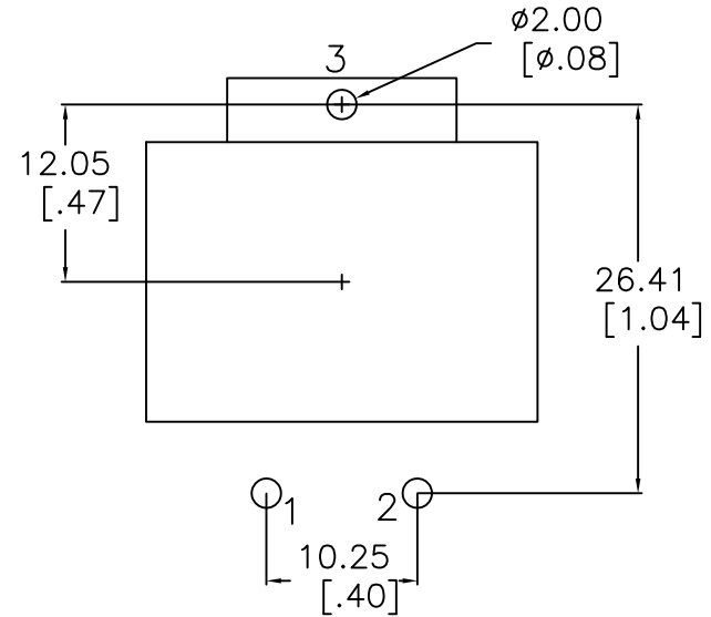
SUGGESTED THRU-HOLE LAYOUT
